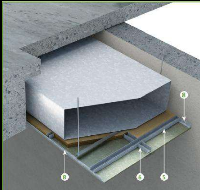
One Sided Duct
