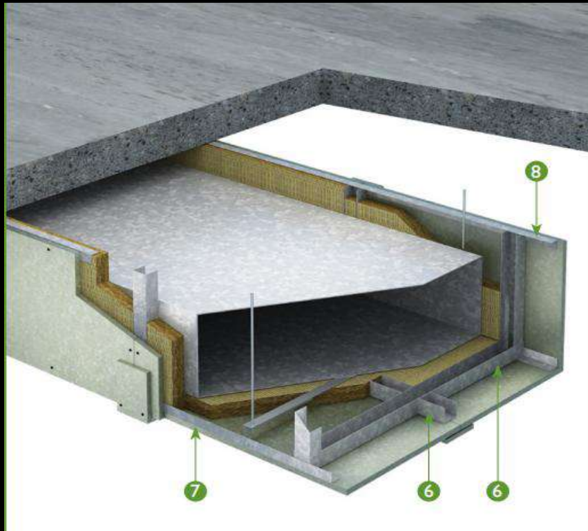
Three Sided Duct
