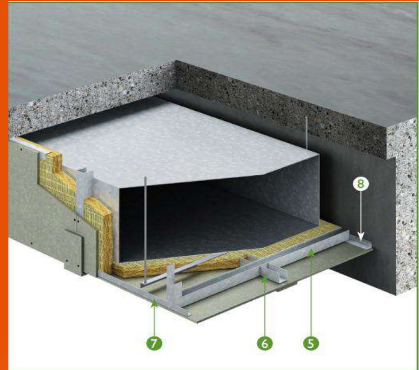
Two Sided Duct
