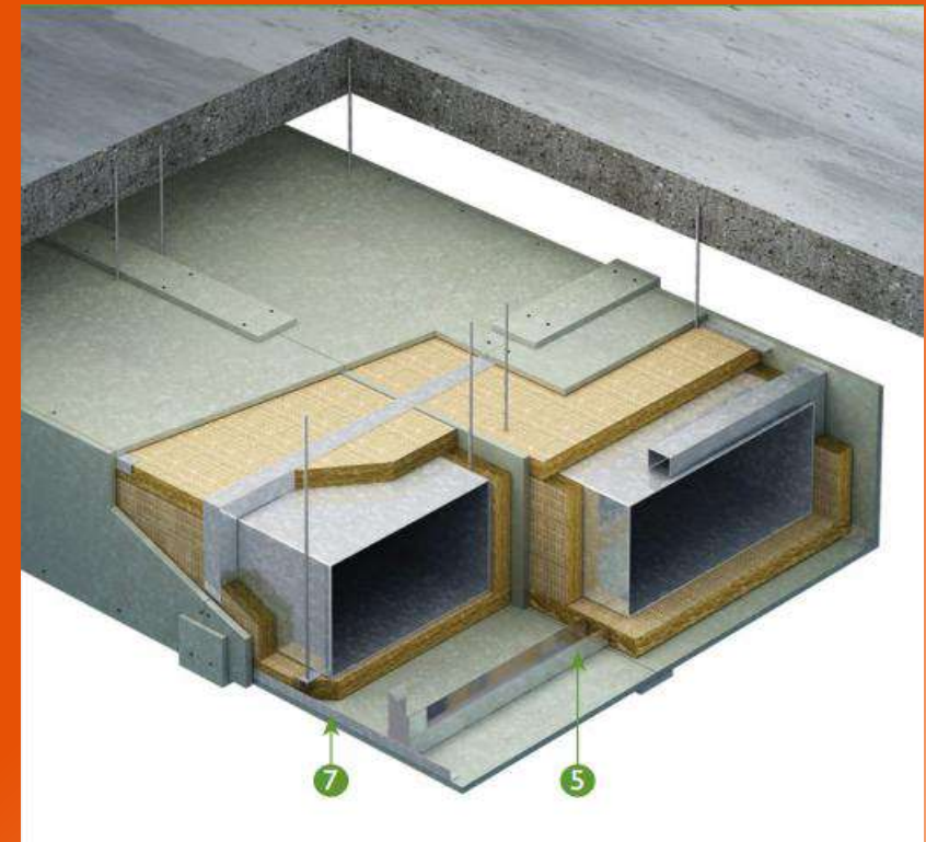
Multiple Side By Side Ducts
